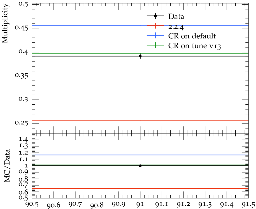
Mean \Lambda multiplicity
