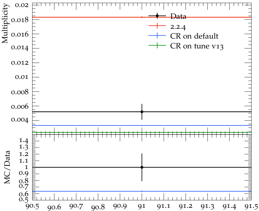
Mean D_{s1}^+ multiplicity
