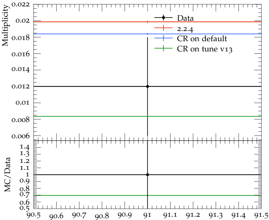
Mean f_2(1525) multiplicity
