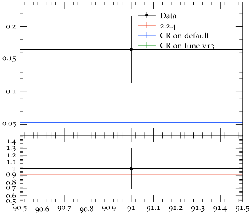
Mean f_1(1285) multiplicity
