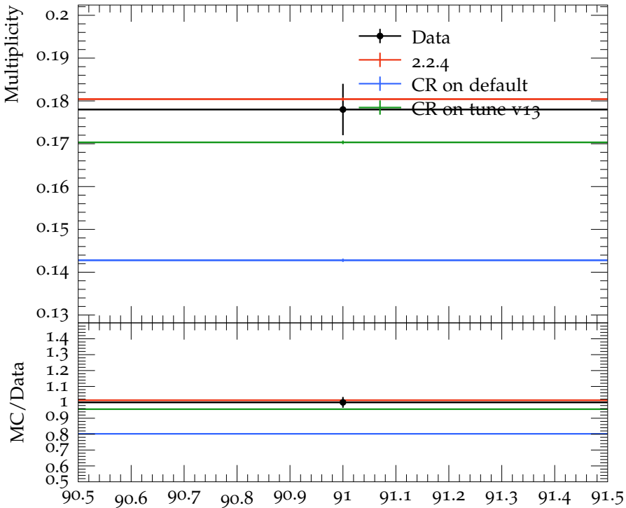
Mean B_u^+ multiplicity
