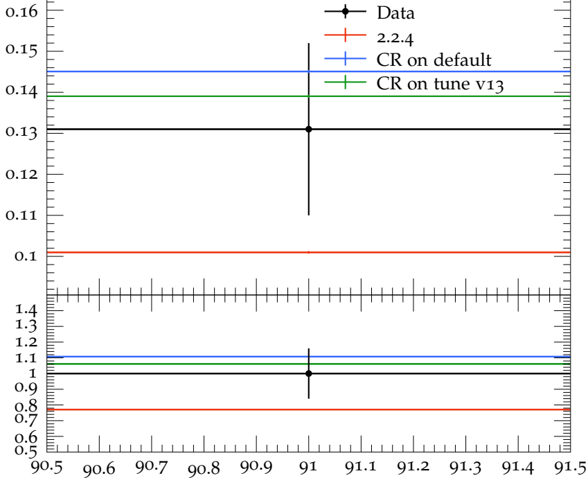
Mean D^+s multiplicity
