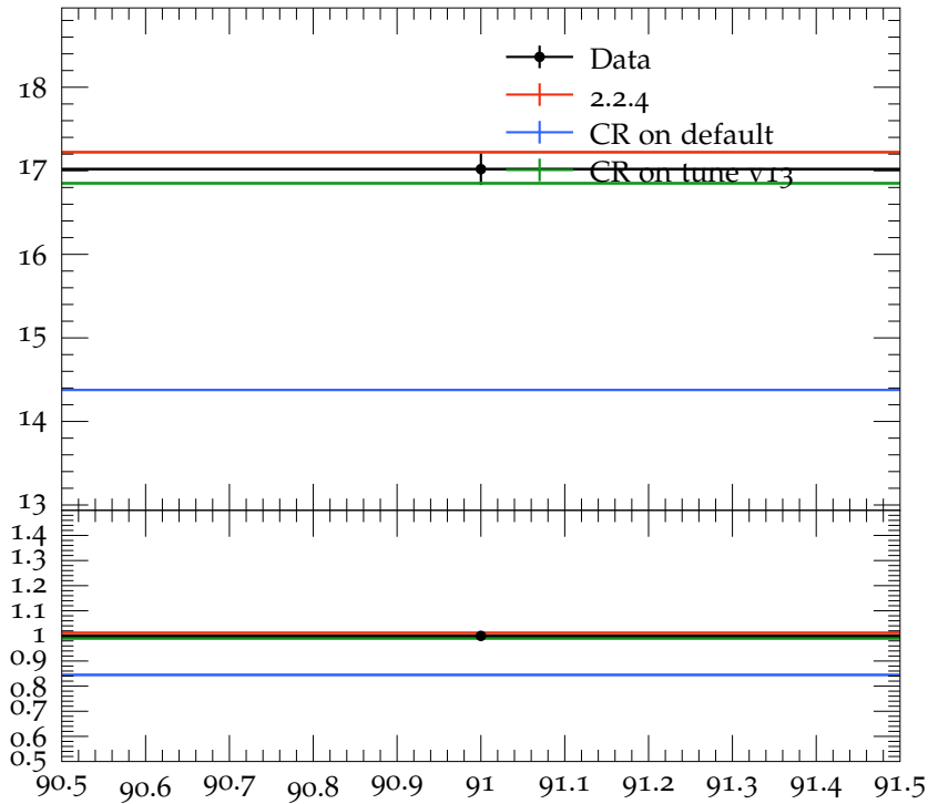
Mean \pi^+ multiplicity
