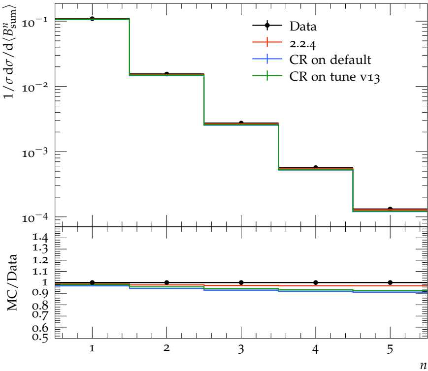
Moments of B_{\text{sum}} at 91 GeV
