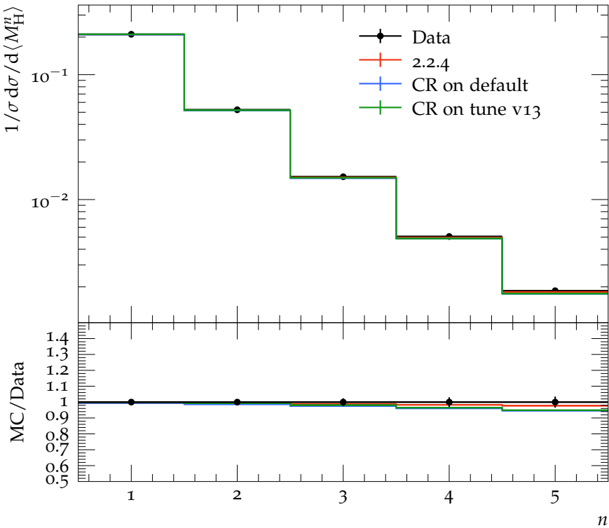
Moments of M_H at 91 GeV
