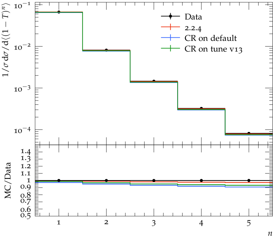
Moments of 1 - T at 91 GeV
