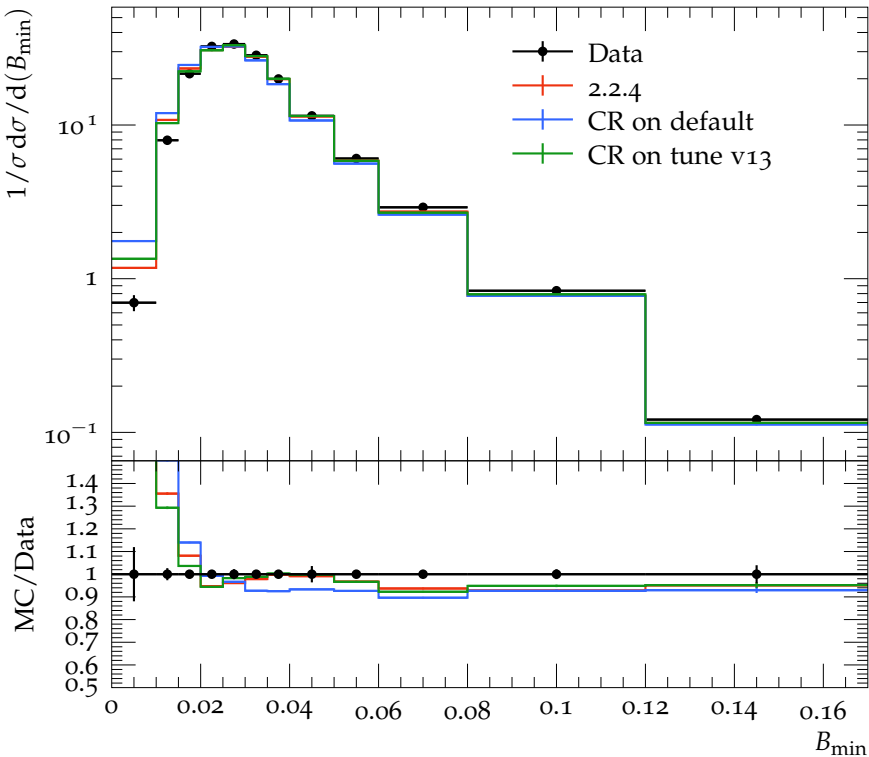
Narrow hemisphere broadening, B_{\min} , at 91 GeV
