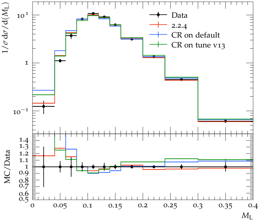
Light hemisphere mass, M_L , at 91 GeV
