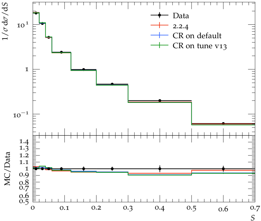
Sphericity, S , at 91 GeV
