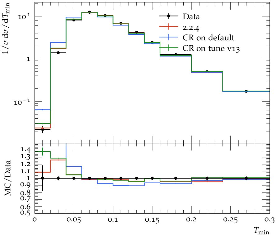
Thrust minor, T_{\min} , at 91 GeV
