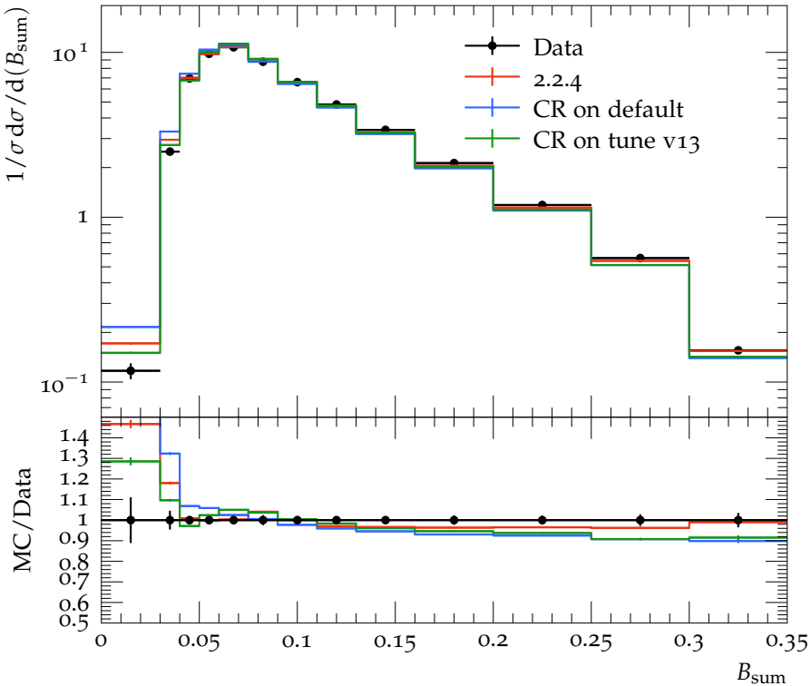
Total hemisphere broadening, B_{\text{sum}} , at 91 GeV
