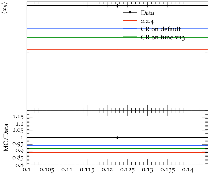
Mean of the b -quark fragmentation function f(x_B^{weak})
