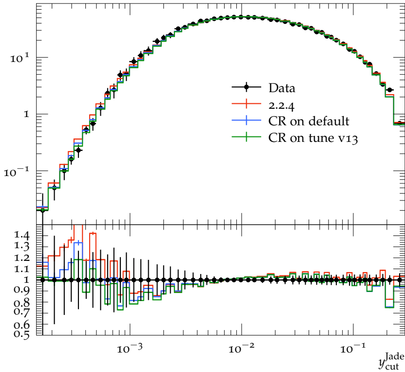
Integrated 3-jet rate with Jade algorithm (91.2 GeV)
