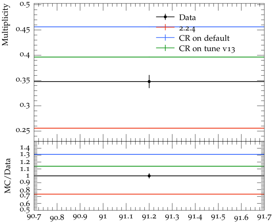
Mean \Lambda^0 multiplicity
