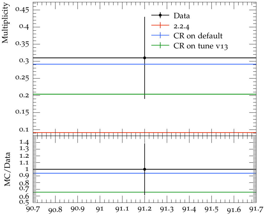
Mean f_2(1270) multiplicity
