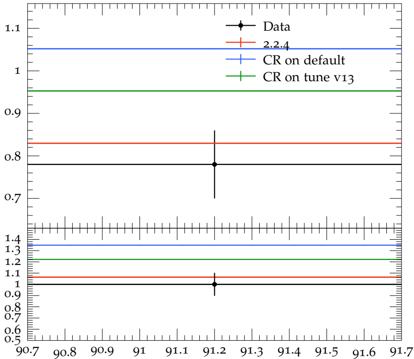
Mean K^*(892)^+ / K^*(892)^- multiplicity
