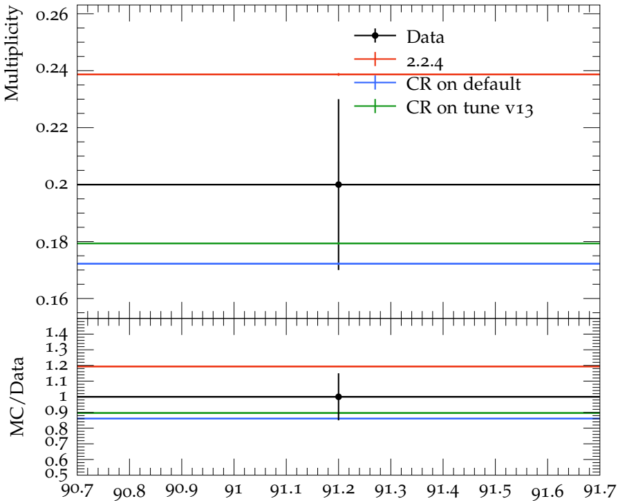
Mean D^+ multiplicity
