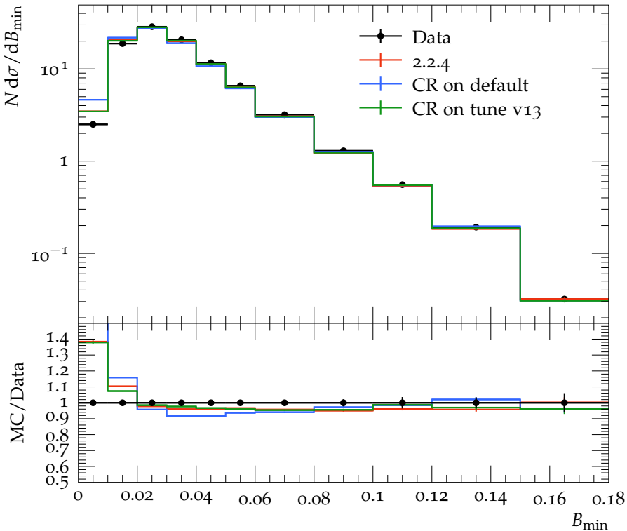
Narrow hemisphere broadening, B_{\min}
