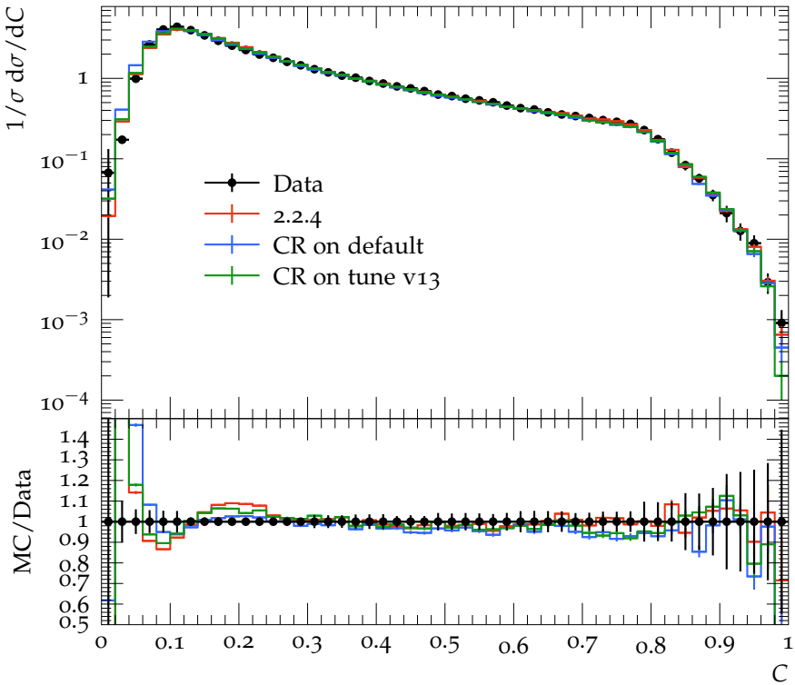
C-Parameter ( E_{\text{CMS}} = 91.2 \text{ GeV} )
