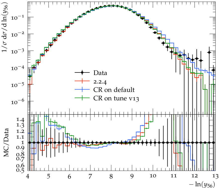
Durham jet resolution 6 \rightarrow 5 ( E_{\text{CMS}} = 91.2 GeV)
