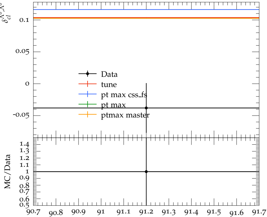
Multiplicity difference b - uds for \Lambda^0, \bar{\Lambda}^0
