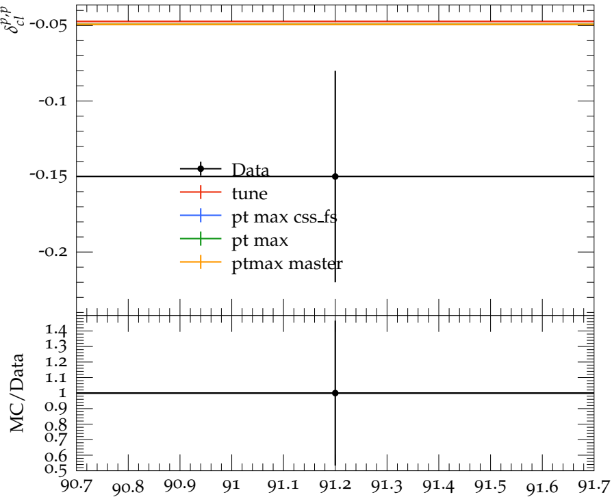
Multiplicity difference b -uds for p, \bar{p}
