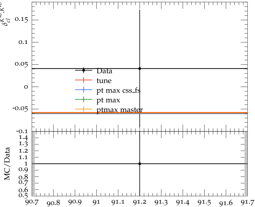
Multiplicity difference b - uds for K^{*0}, \bar{K}^{*0}
