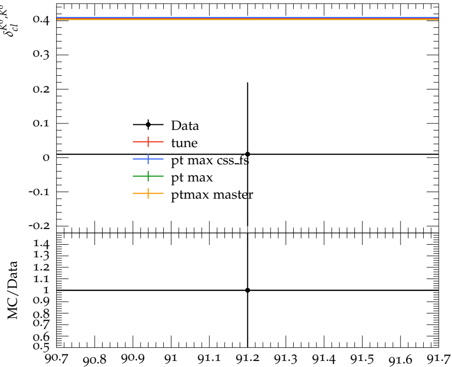
Multiplicity difference c -uds for K^0, \bar{K}^0
