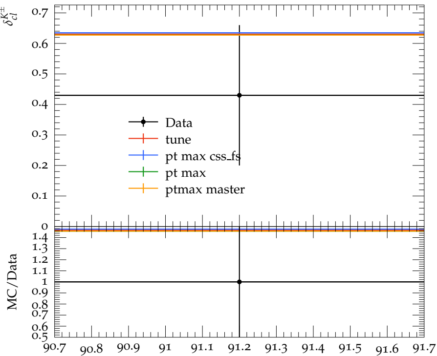
Multiplicity difference c - uds for K^\pm
