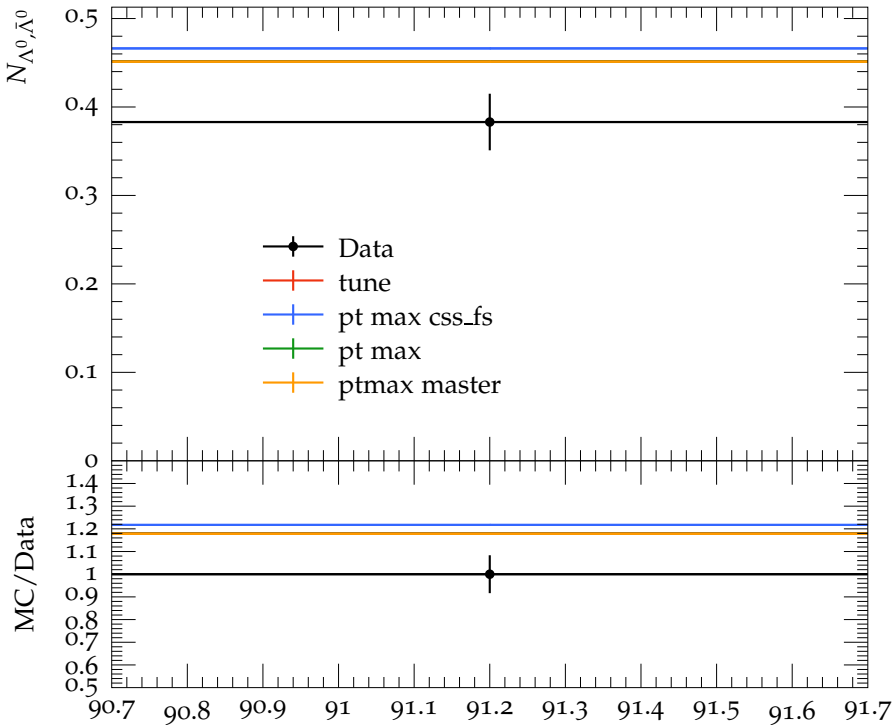
Multiplicity of \Lambda^0, \bar{\Lambda}^0 in b events
