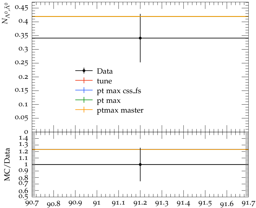
Multiplicity of \Lambda^0, \bar{\Lambda}^0 in c events
