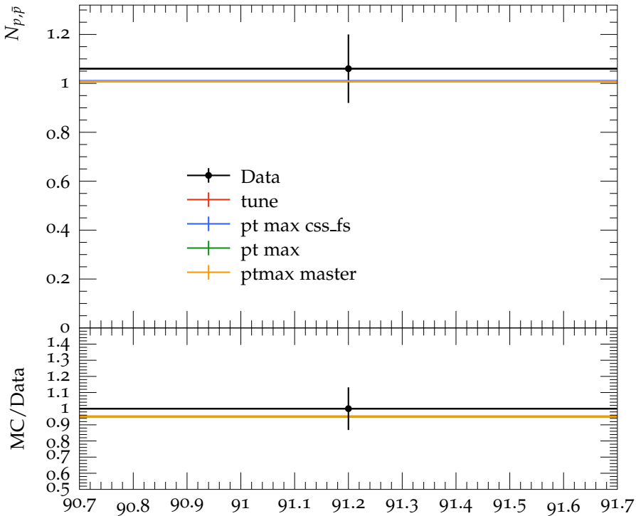
Multiplicity of p, \bar{p} in ( uds ) events
