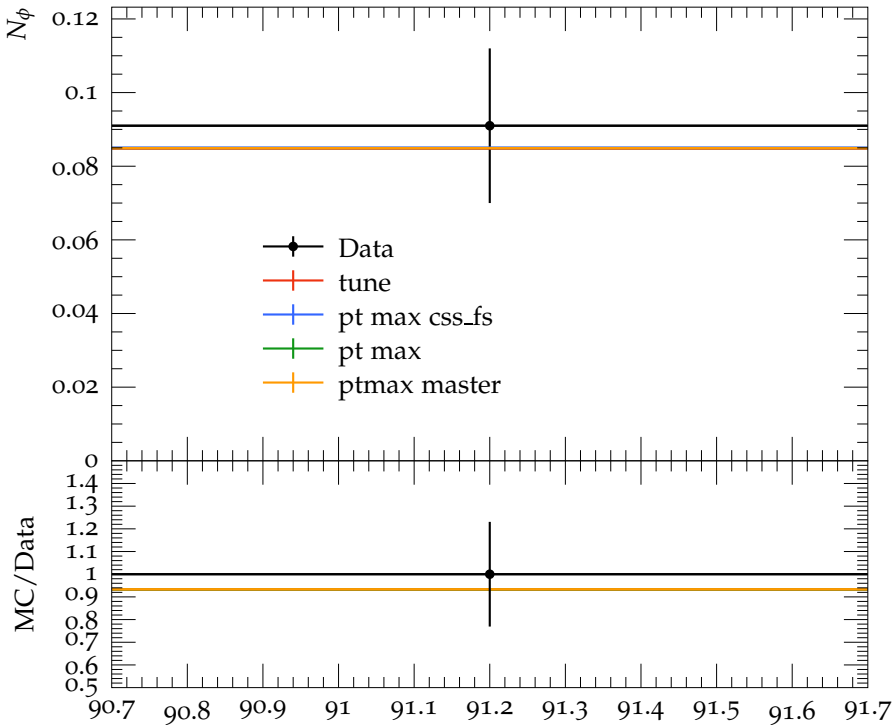
Multiplicity of \phi in ( uds ) events
