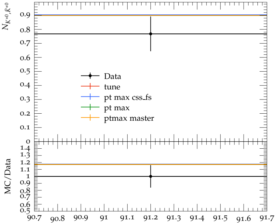
Multiplicity of K^{*0}, \bar{K}^{*0} in b events
