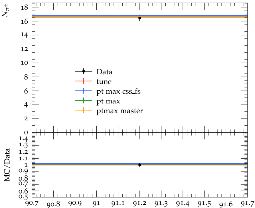
Multiplicity of \pi^\pm in ( uds ) events
