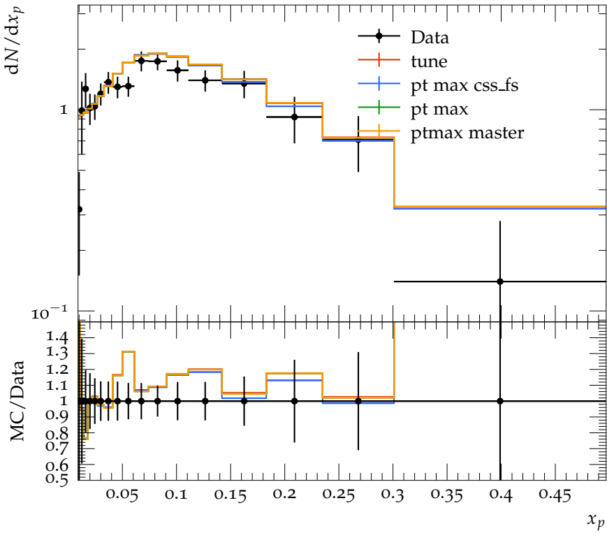
K^0 scaled momentum, ratio b to uds events
