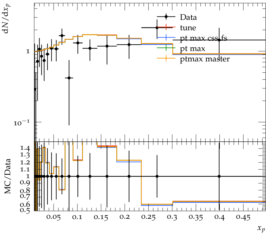
K^0 scaled momentum, ratio c to uds events
