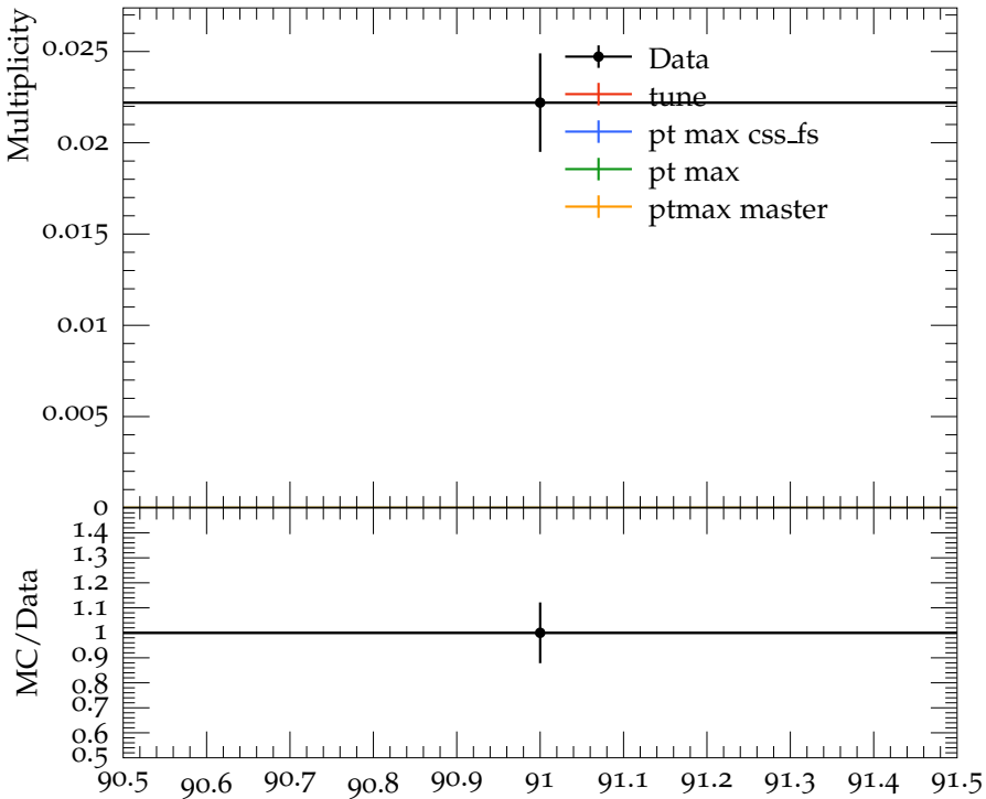
Mean \Lambda(1520) multiplicity
