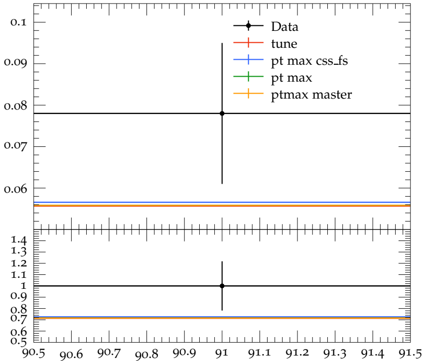
Mean \Lambda_c^+ multiplicity
