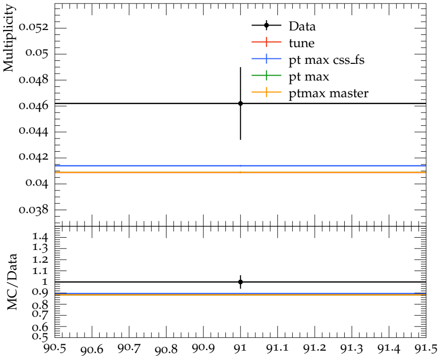
Mean \Sigma^\pm(1385) multiplicity
