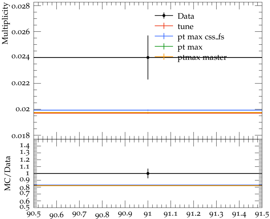
Mean \Sigma^- (1385) multiplicity
