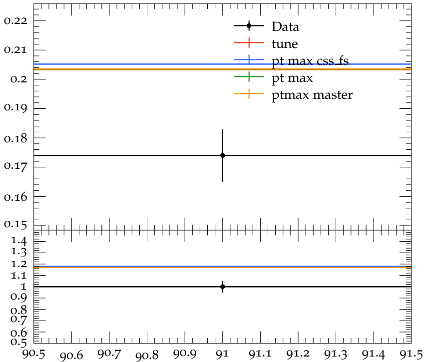
Mean \Sigma^\pm multiplicity
