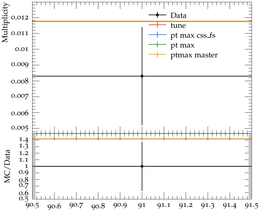
Mean D_{s2}^+ multiplicity
