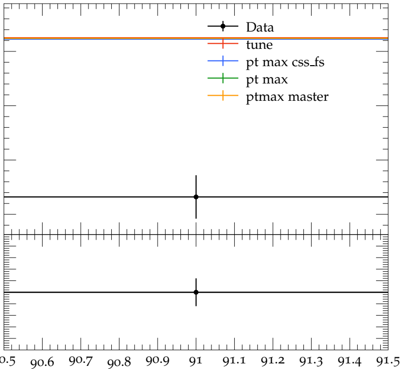
Mean f_2(1270) multiplicity
