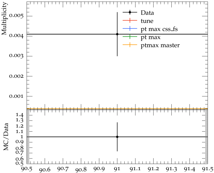
Mean \chi_{c1}(3510) multiplicity
