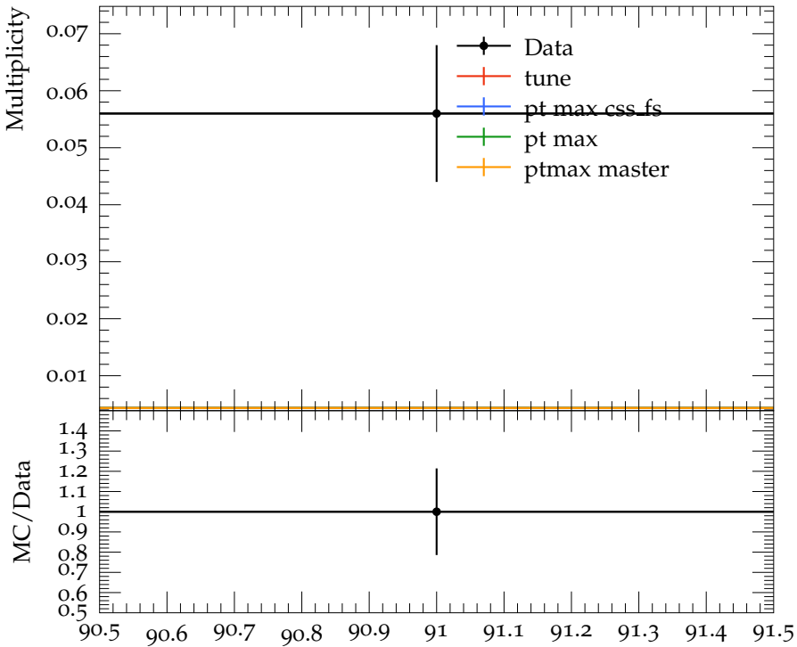
Mean f_1(1420) multiplicity
