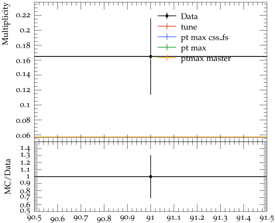
Mean f_1(1285) multiplicity
