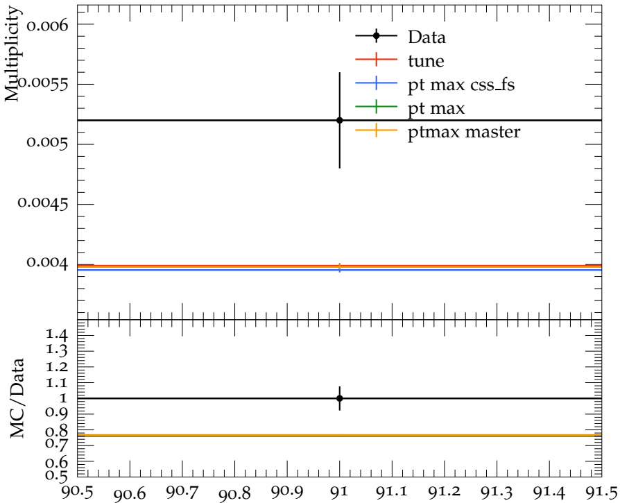
Mean J/\psi(1S) multiplicity
