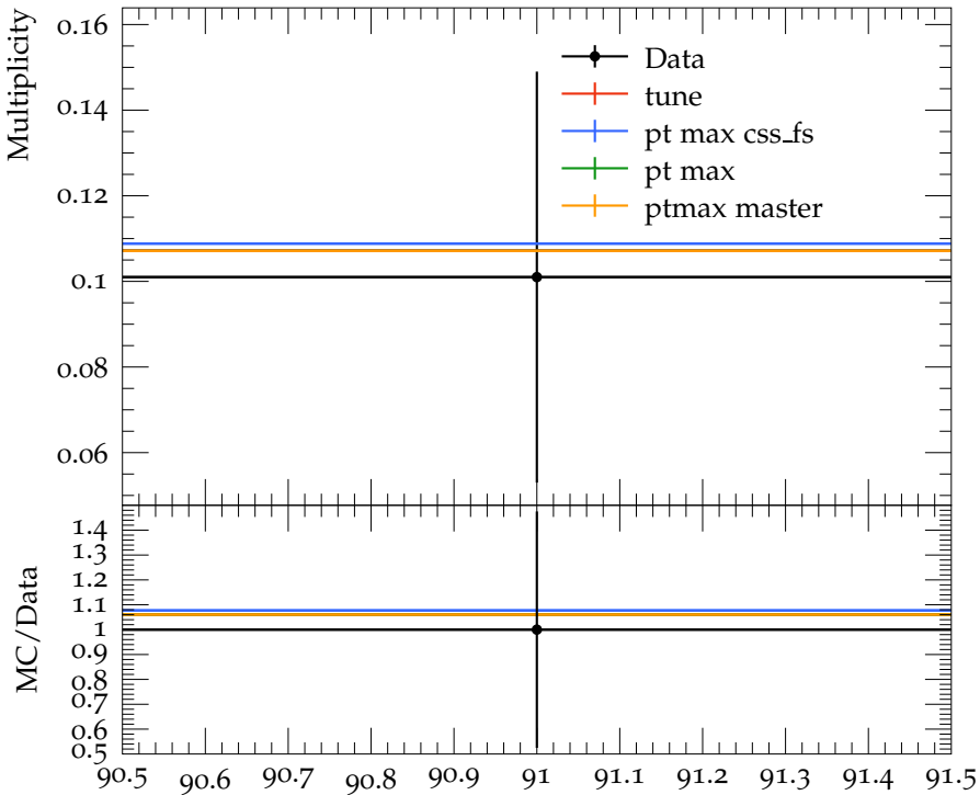
Mean D_s^{*+}(2112) multiplicity
