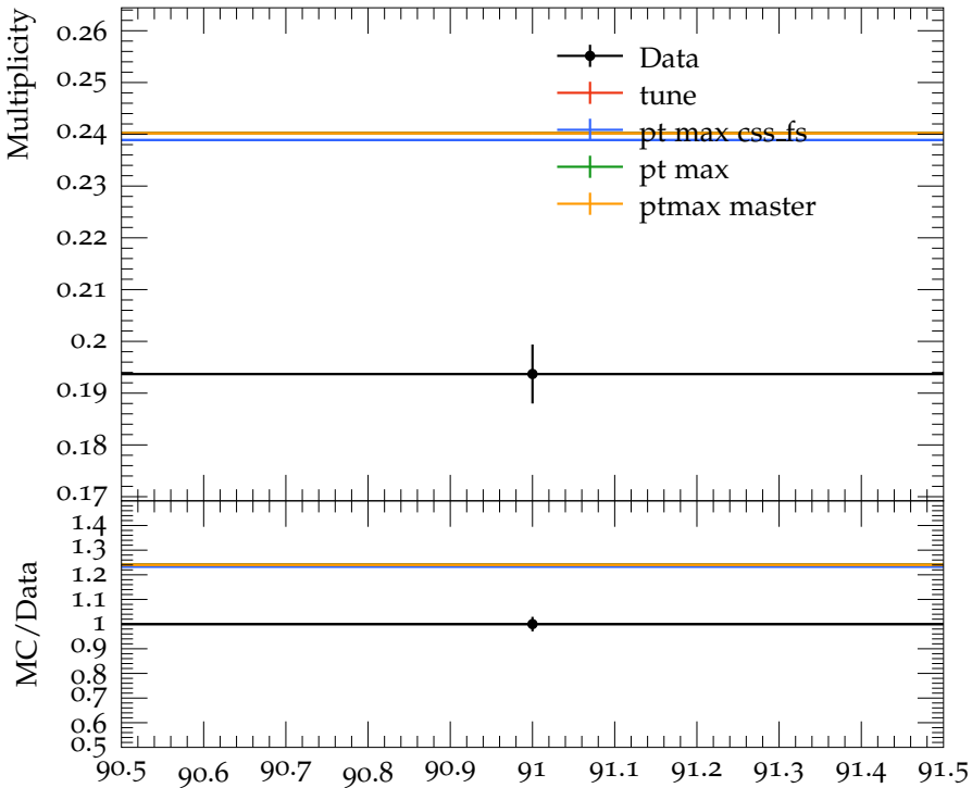
Mean D^{*+} (2010) multiplicity
